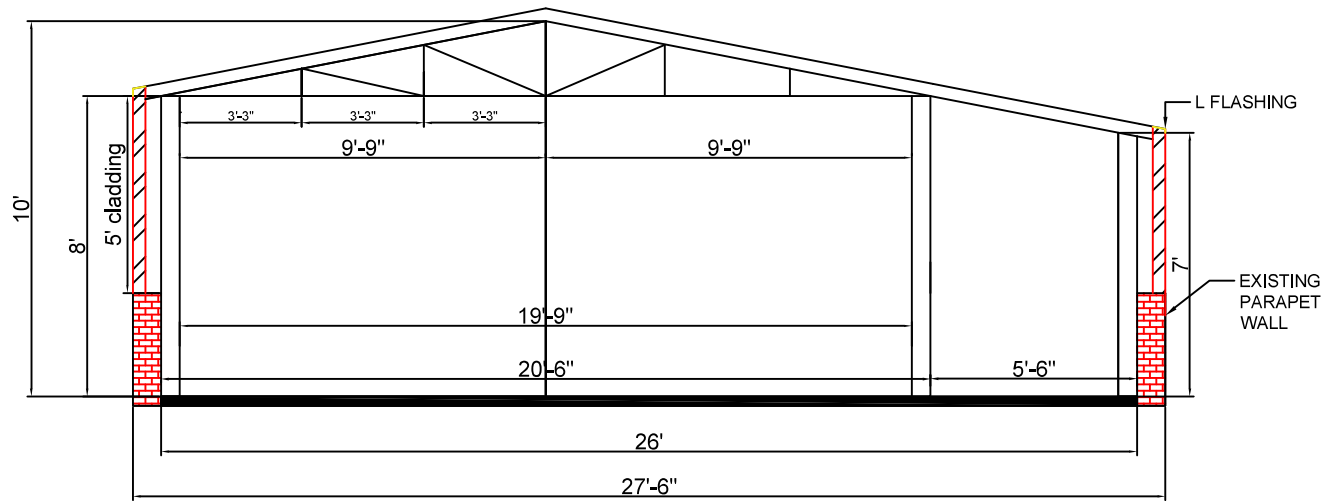
CROSS SECTION OF GI ROOFING FOR GIRLS HOSTEL TERRACE
