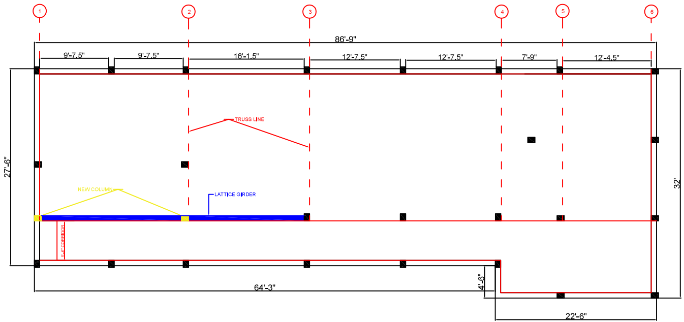
TITLE : PLAN FOR GIRLS HOSTEL
